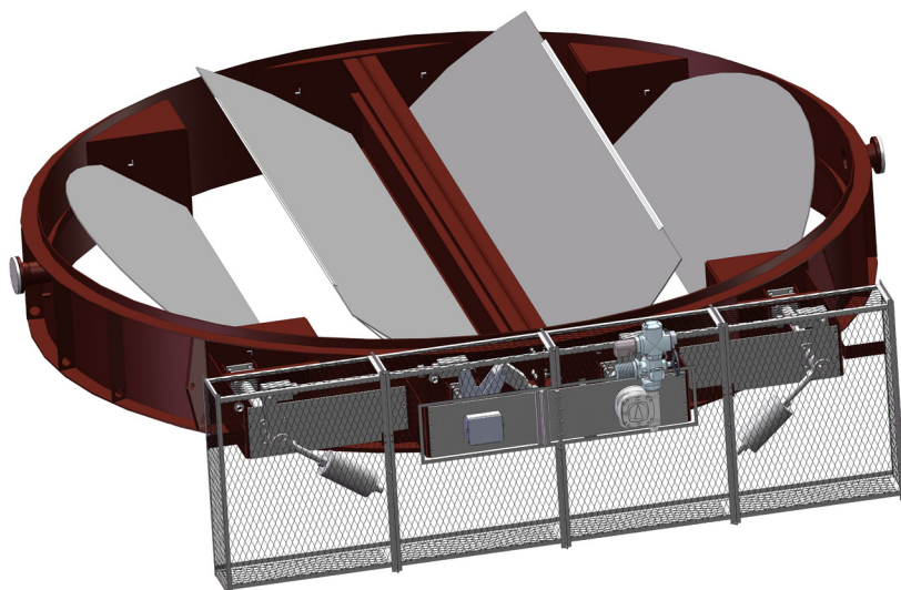
Custom stack damper with guards around linkages.
